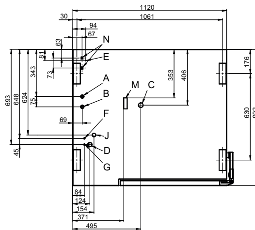
Connection points
