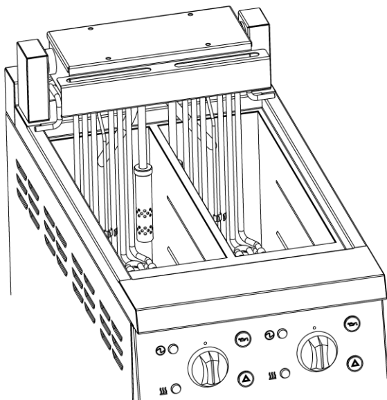
Oil level sensor guard lowered.
