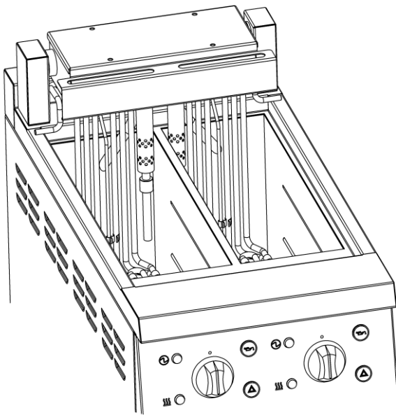
Oil level sensor guard raised for cleaning.
