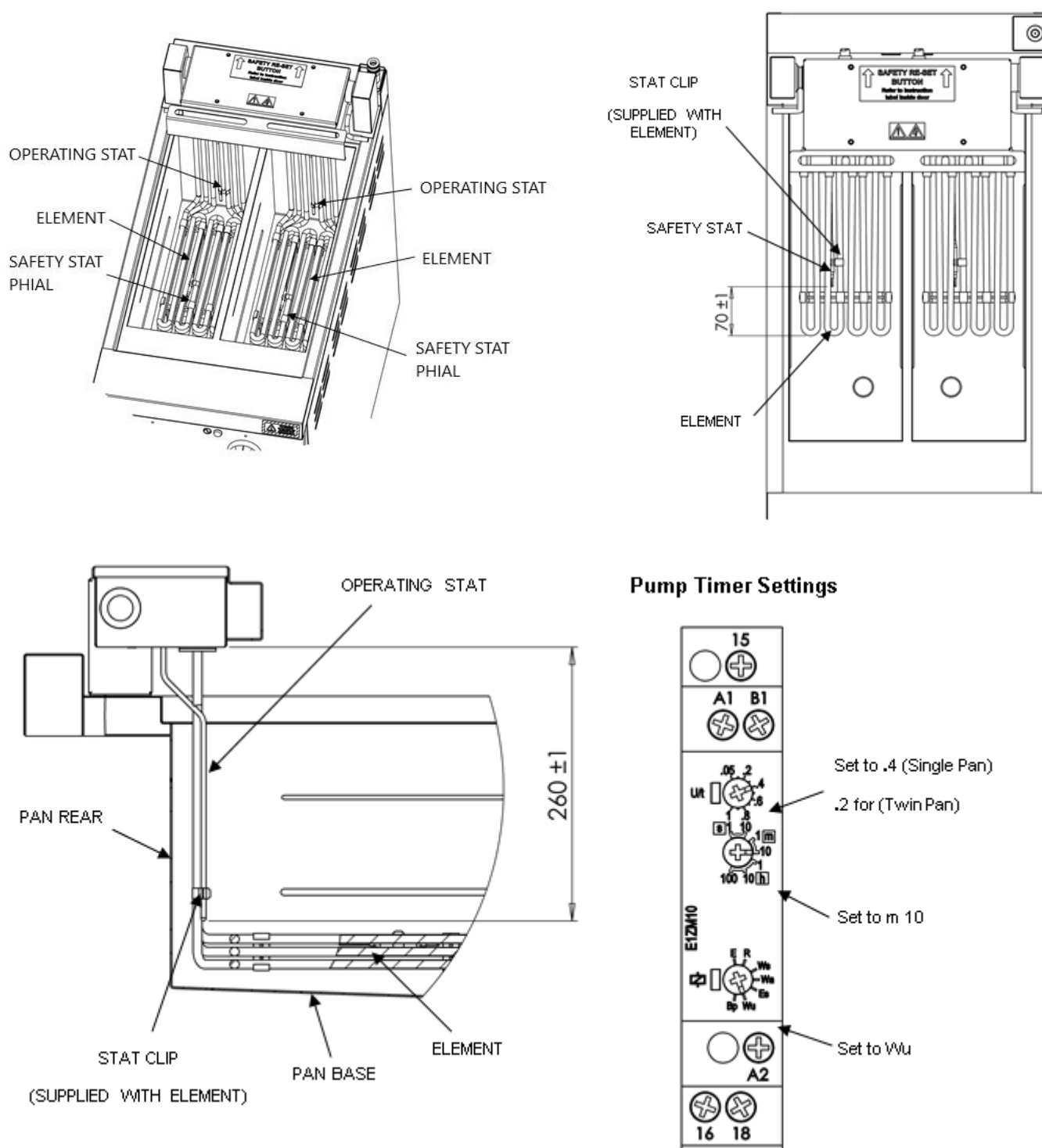
Figure 9 – Critical dimensions
