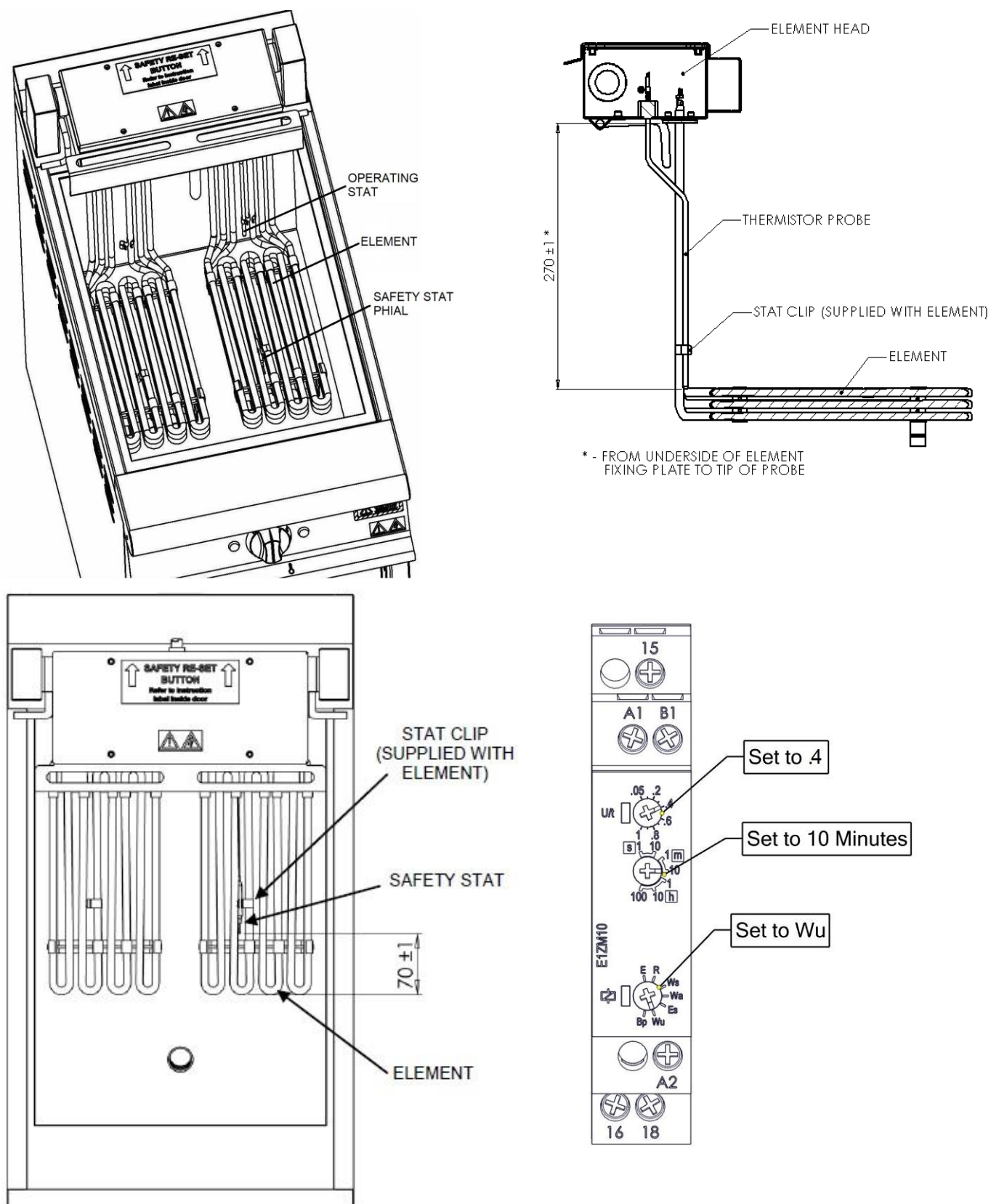
Figure 9 – Critical Dimensions
