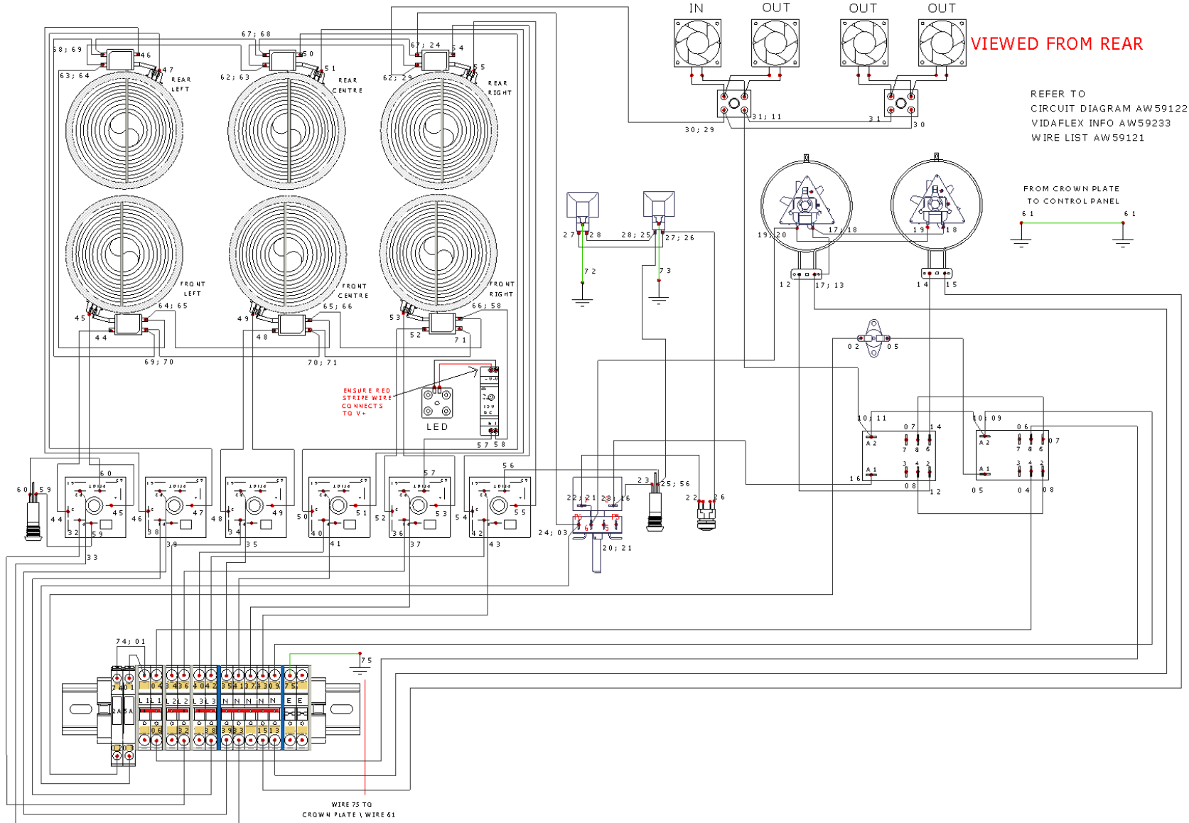
E3164 WIRING DIAGRAM (MAIN)
